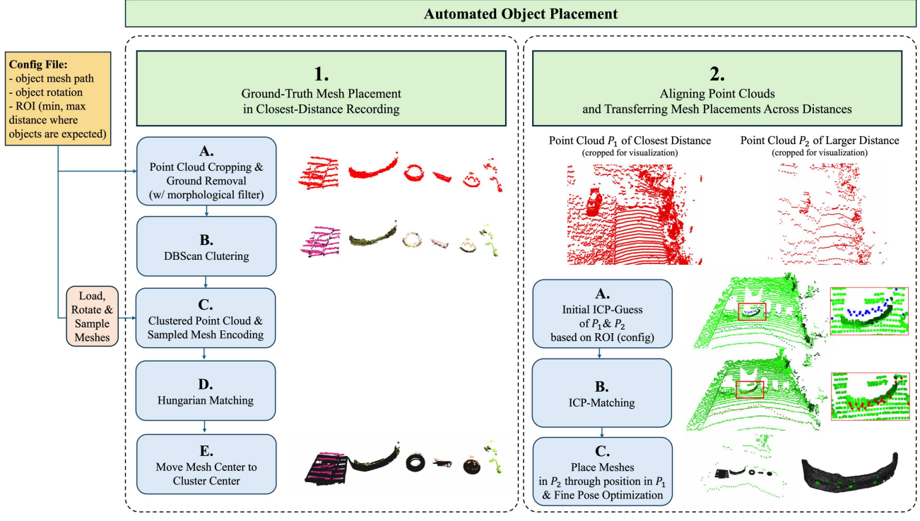
Figure 1. Automated Object Placement. Overview of the two-stage process: stage one places the ground-truth mesh in the recording with the closest distance, and stage two applies this placement to all other distances and sensors.
