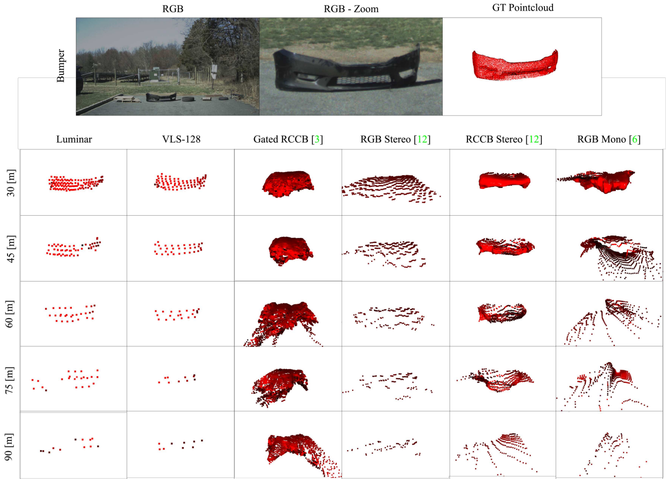
Figure 9. Summer Recording: Bumper. Visual results of lost cargos captured at different distances, with different depth estimation methods, comprising cross spectral Gated RCCB fusion [3], RGB Stereo [12], RCCB Stereo [12] and RGB Monocular [6], and LiDAR sensors from Luminar and Velodyne.
