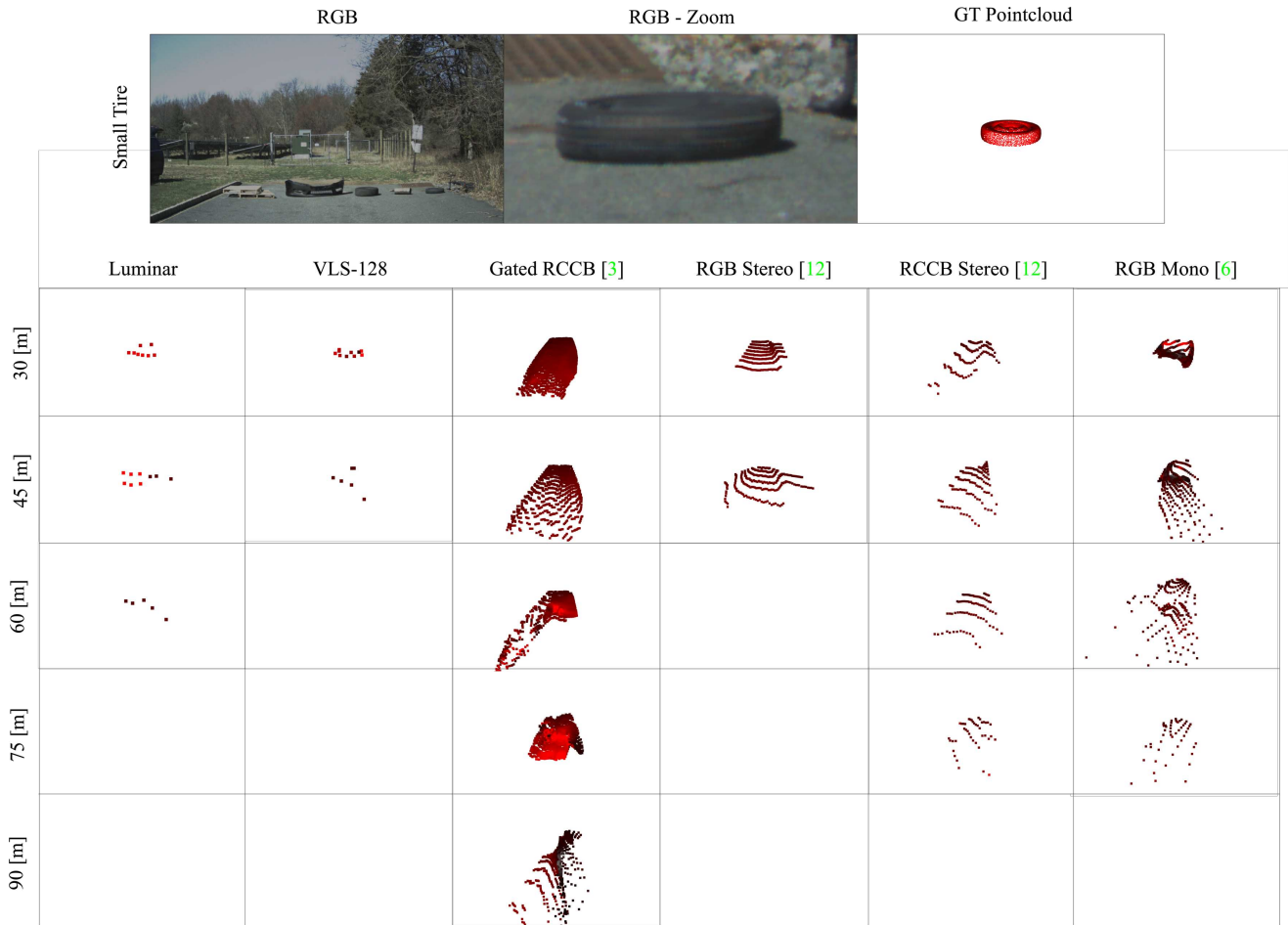
Figure 12. Summer Recording: Small Tire. Visual results of lost cargos captured at different distances, with different depth estimation methods, comprising cross spectral Gated RCCB fusion [3], RGB Stereo [12], RCCB Stereo [12] and RGB Monocular [6], and LiDAR sensors from Luminar and Velodyne.
