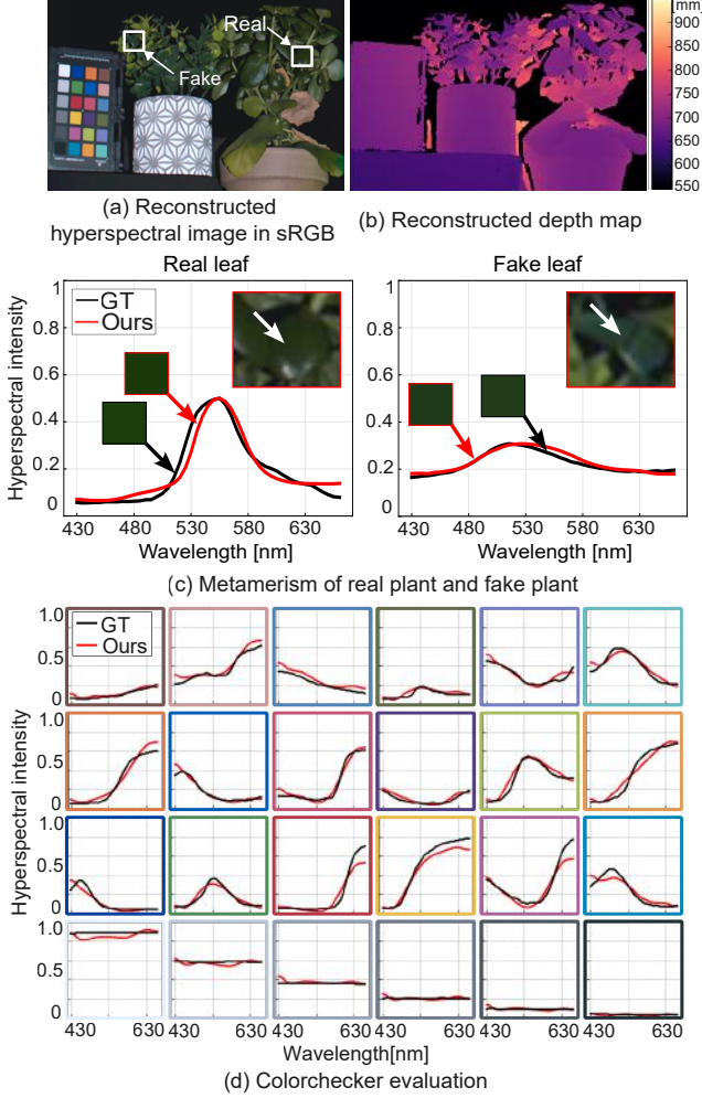
Figure 8. Evaluation on a ColorChecker and metamerics samples. (a) Reconstructed hyperspectral image in sRGB, (b) reconstructed depth map, (c) spectra of metamerics samples (real and fake leaves), (d) reconstructed spectra of each color patch.
