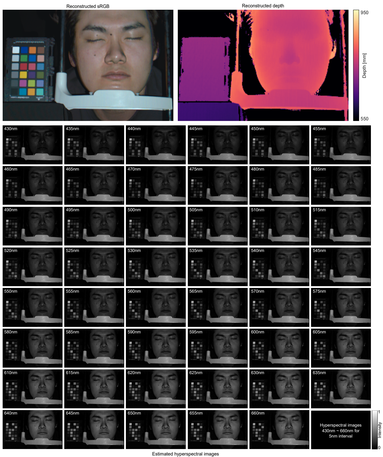
Figure 11. Hyperspectral 3D imaging. We show the result of a face scanned reconstructed hyperspectral image in sRGB, reconstructed depth and the detailed hyperspectral image for 5 nm interval.
