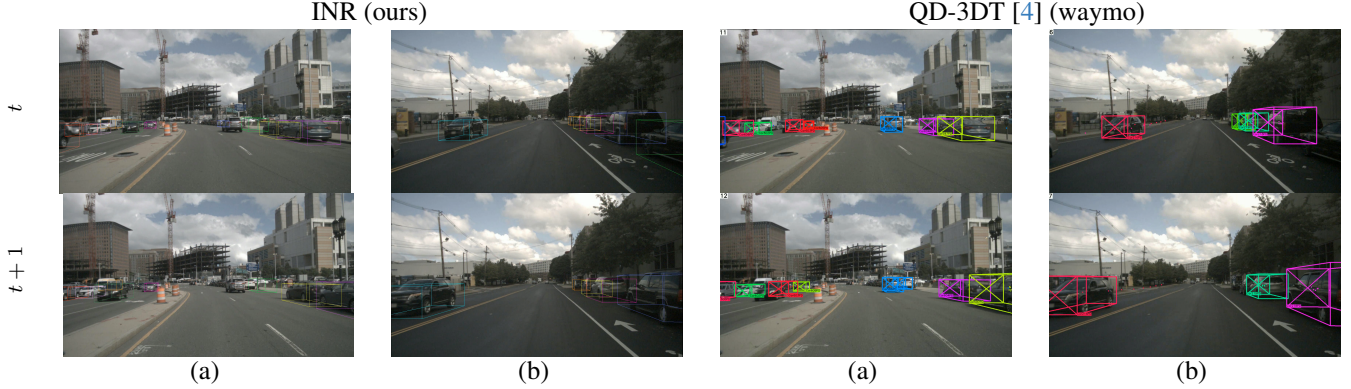
Figure 3. Qualitative Comparison on Generalization. We compare 3D bounding box outputs from QD-3DT [4] trained on waymo [12] and our inverse neural rendering based tracker (INR) overlayed on the respective input videos from nusenes [1]. The same color in consecutive frames denote same tracklet. As we see in scene (a) on the left side QD-3DT is having ID switches especially in the far range and on the sides of a frame implying dataset specific performance caps, e.g. the training dataset has been tracking annotated in a rather short range. Another finding is exemplified in scene (b) on the right side where the tracker does not generalize well and is losing a tracklet.
