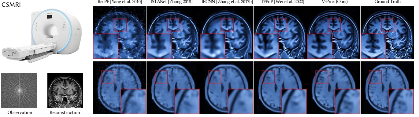
Fig. 7. Qualitative comparisons of CS-MRI reconstruction for human brain scans. The predictions of ∇-Prox correspond to "Learning Scheduler for DRUNet" in Table 3. Using a PnP prior (DRUNet) and an RL-based parameter selection policy, the trained solver output from ∇-Prox achieves unprecedented reconstruction quality compared to state-of-the-art methods. For example, it precisely recovers the cerebral ravine and brain tissues that are inaccurately reconstructed or totally missed in other methods.
