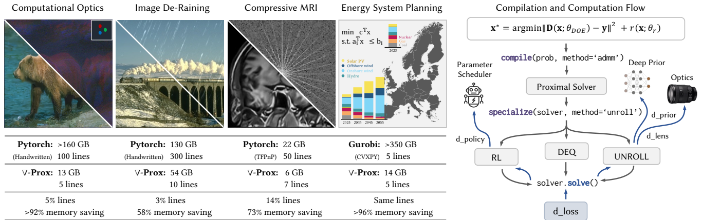
Fig. 1. ∇-Prox is a domain-specific language (DSL) and compiler that transforms optimization problems into differentiable proximal solvers. Departing from handwriting these solvers and differentiating via autograd, ∇-Prox requires only a few lines of code to define a solver that can be specialized to respect a memory or training budget by optimized algorithm unrolling, deep equilibrium learning, and deep reinforcement learning. ∇-Prox allows for rapid prototyping of learning-based bi-level optimization problems for a diverse range of applications. We compare our framework against existing methods with naive implementations. ∇-Prox is significantly more compact in terms of lines of code and compares favorably in memory consumption for diverse tasks.
