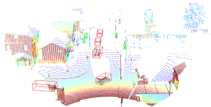
Optimized
