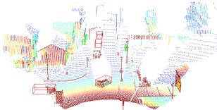
Ground Truth
