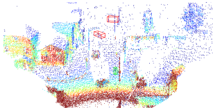
Expert-Tuned
